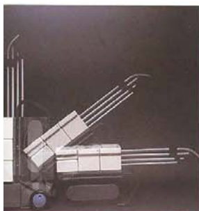
Space saving design: The VersaTile™ system is "user friendly." Tips flip from horizontal operational position to an upright position for space-saving convenience, transport and storage.
